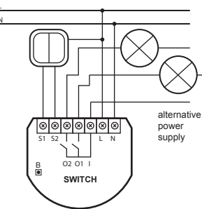
Fig.1 Circuit diagrams for Double Relay Switch.
